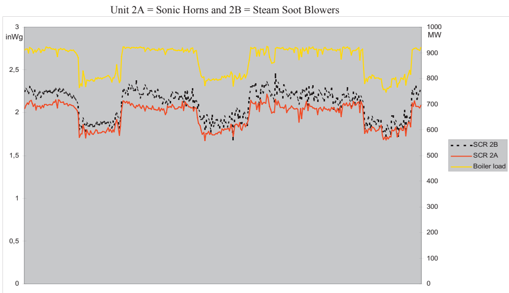
The yellow line is the boiler load The black line is the diff. press with steam soot blowers and the red line is the diff. press with sonic horns.
