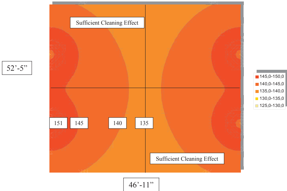
Sound propagation when sound emitter 1+2+3+4 are activated at the same time.
