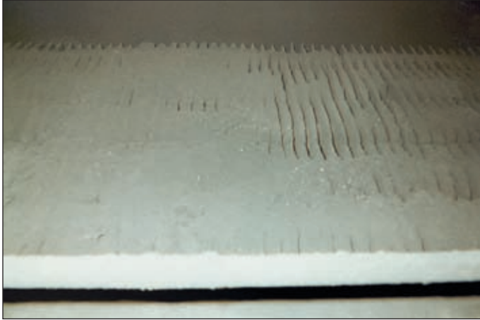
Economizer section, after one month process without Sonic Cleaning. The entire boiler has to be shut down at this time.
