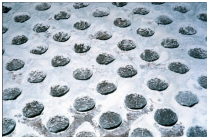
Air preheater, after four months process with Sonic Cleaning.
