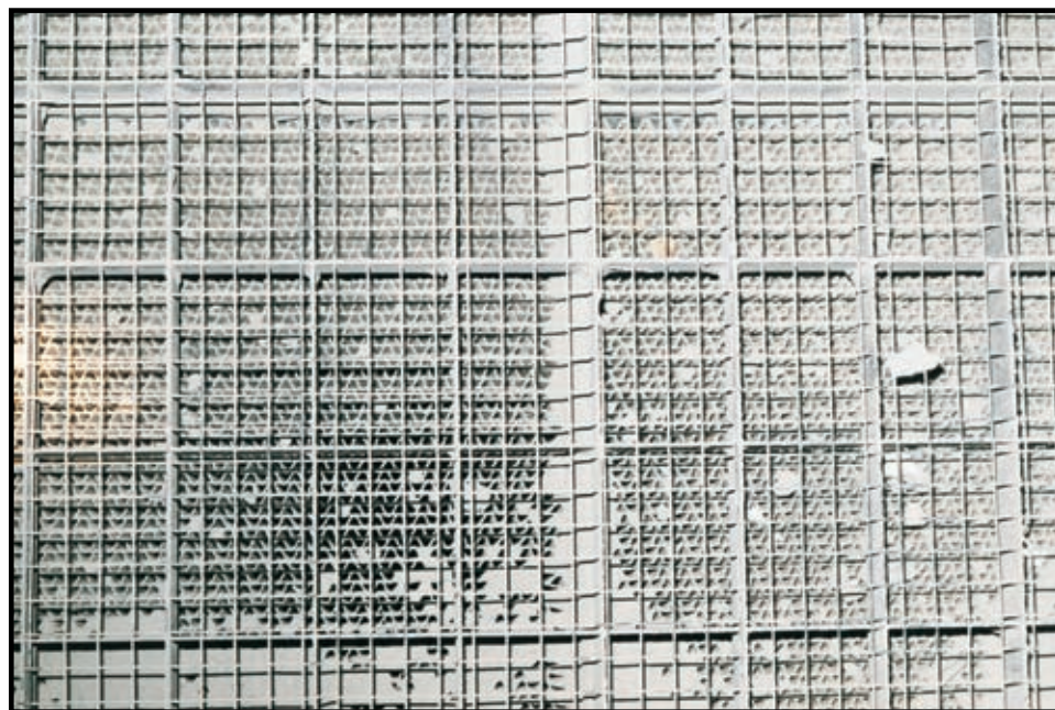
SCR, AFTER SIX MONTHS PROCESS: WITH SONIC CLEANING
