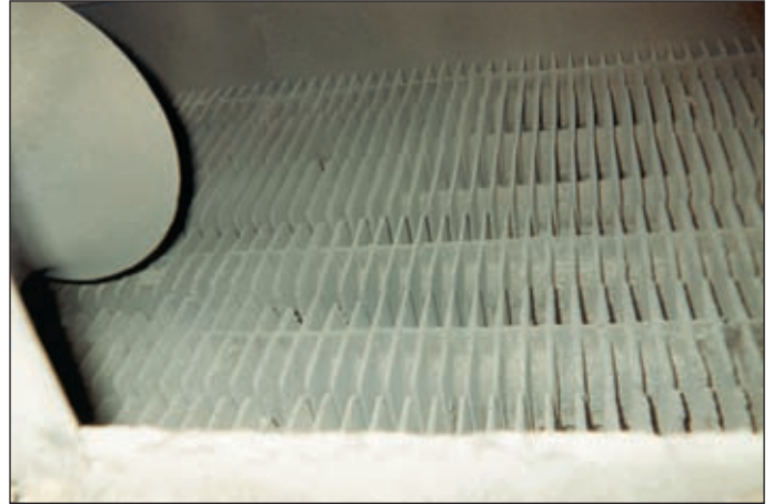
Economizer section, after one month process with Sonic Cleaning.
